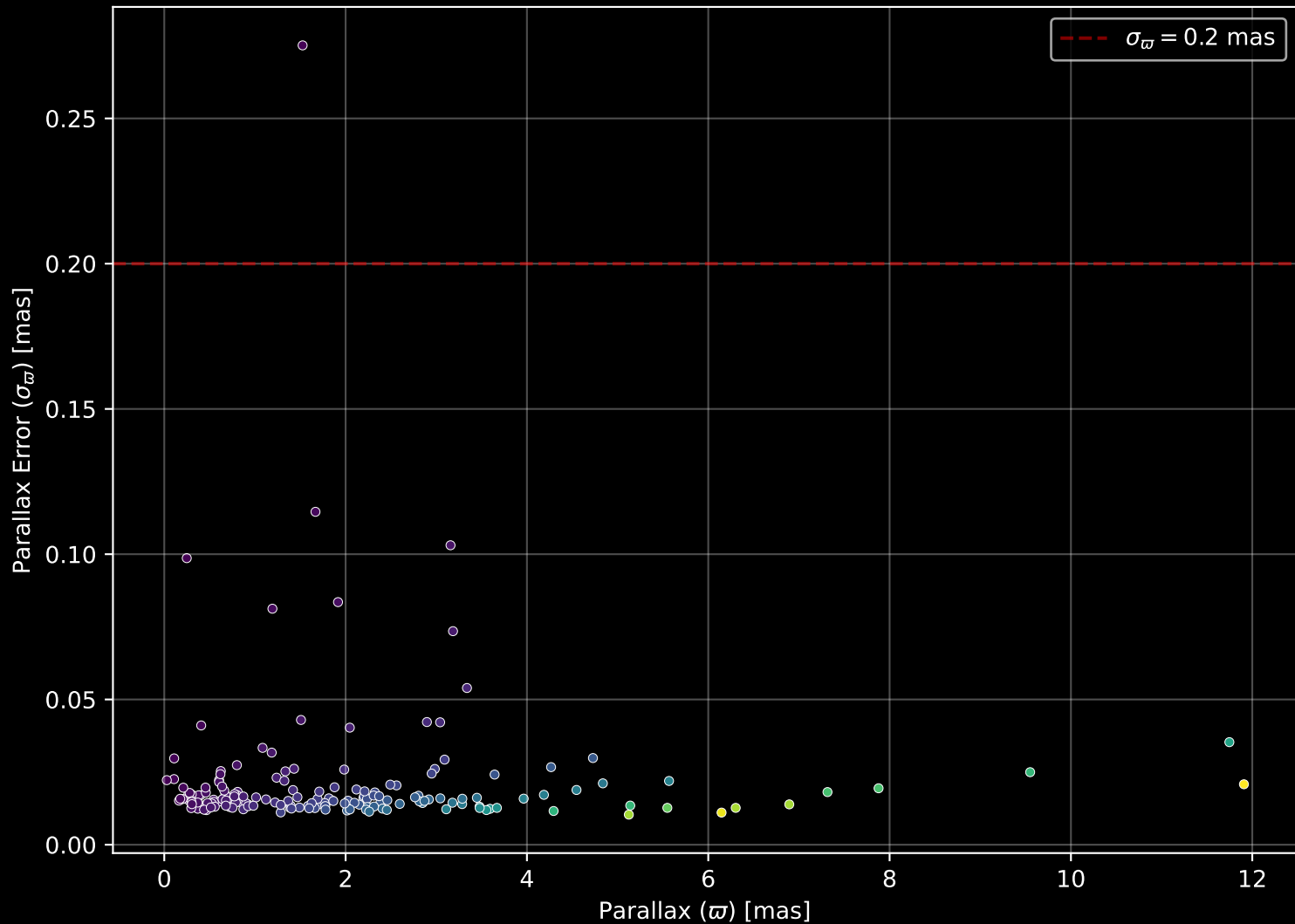
APOGEE DR17 Field: [TRIAND-3] Parallax Quality (n= 174)
