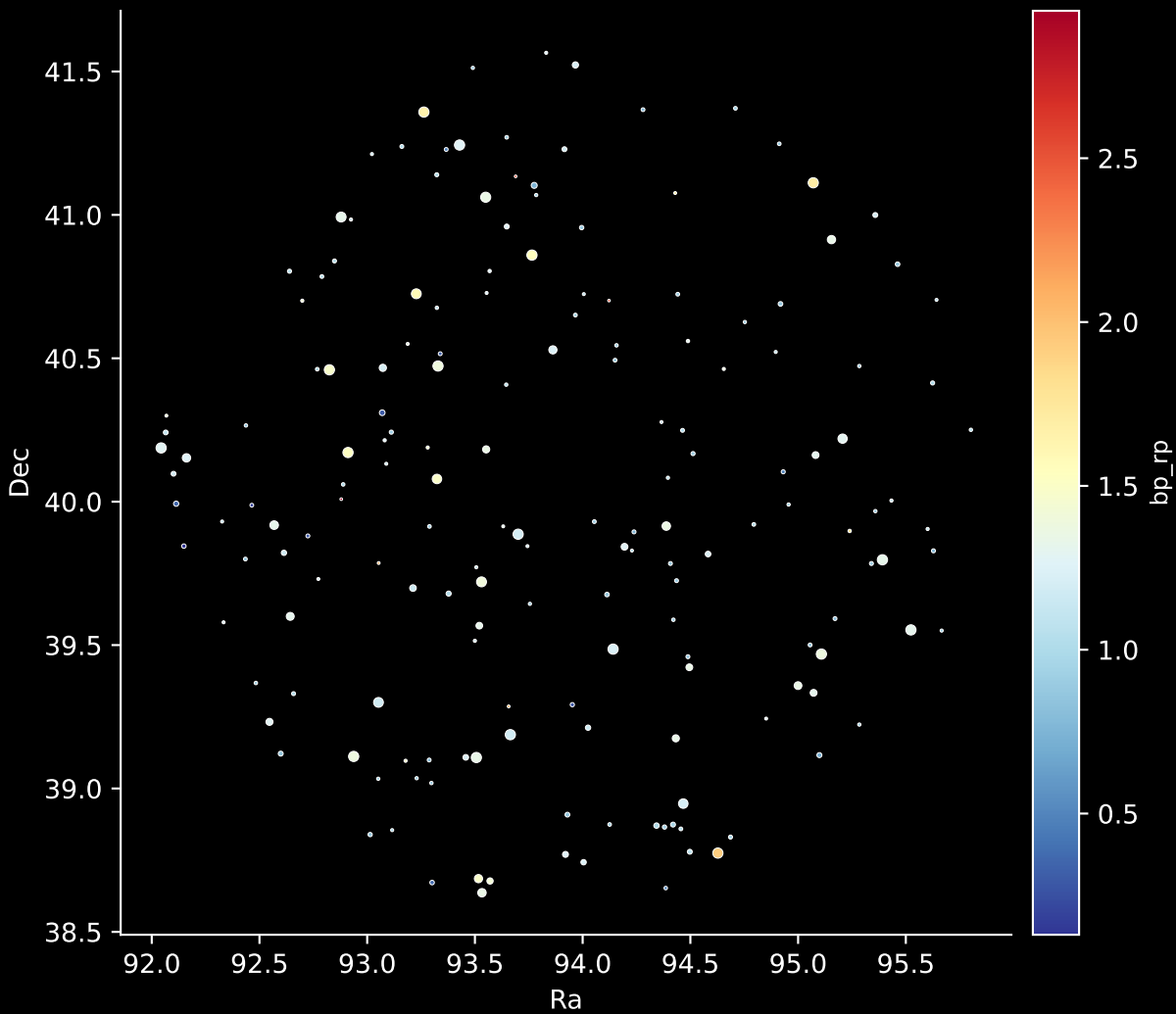
APOGEE DR17 Field: [TRIAND-3] Stars: 174
