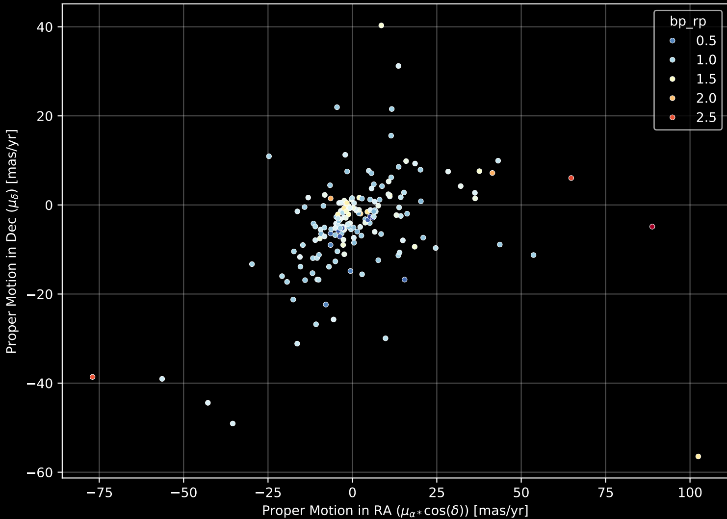
APOGEE DR17 Field: [TRIAND-3] Proper Motion Diagram (n= 174)
