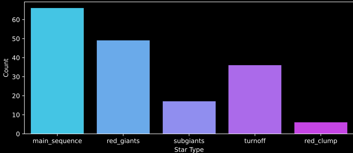
APOGEE DR17 Field: [TRIAND-3] Count plot of Star Type
