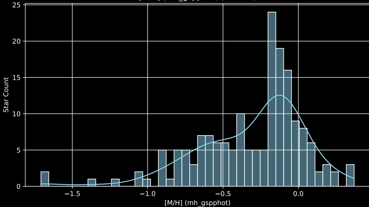
APOGEE DR17 Field: [TRIAND-3 [M/H] (mh_gspphot) (n= 174)
