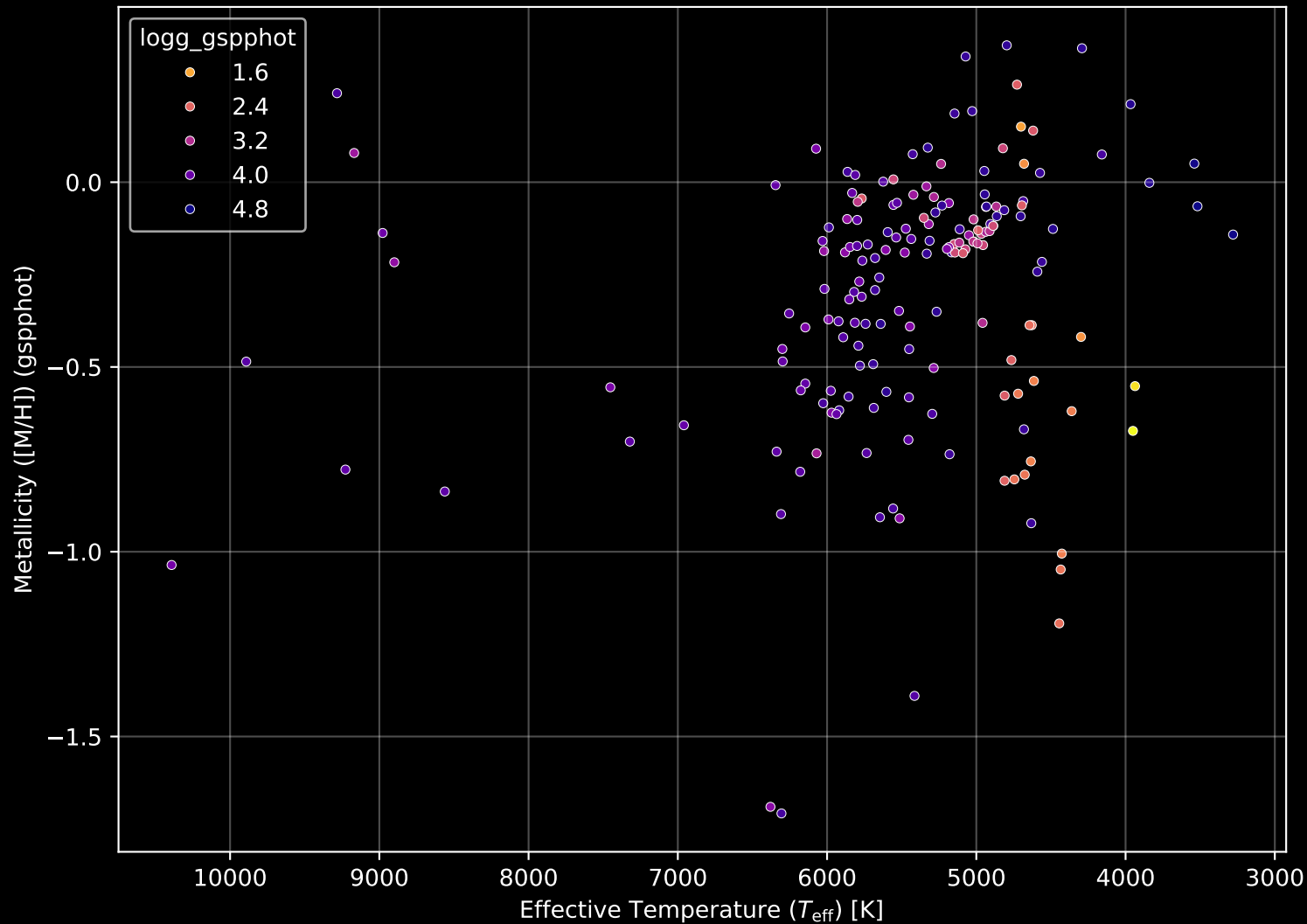
APOGEE DR17 Field: [TRIAND-3] Stellar Population Parameters (n= 174)
