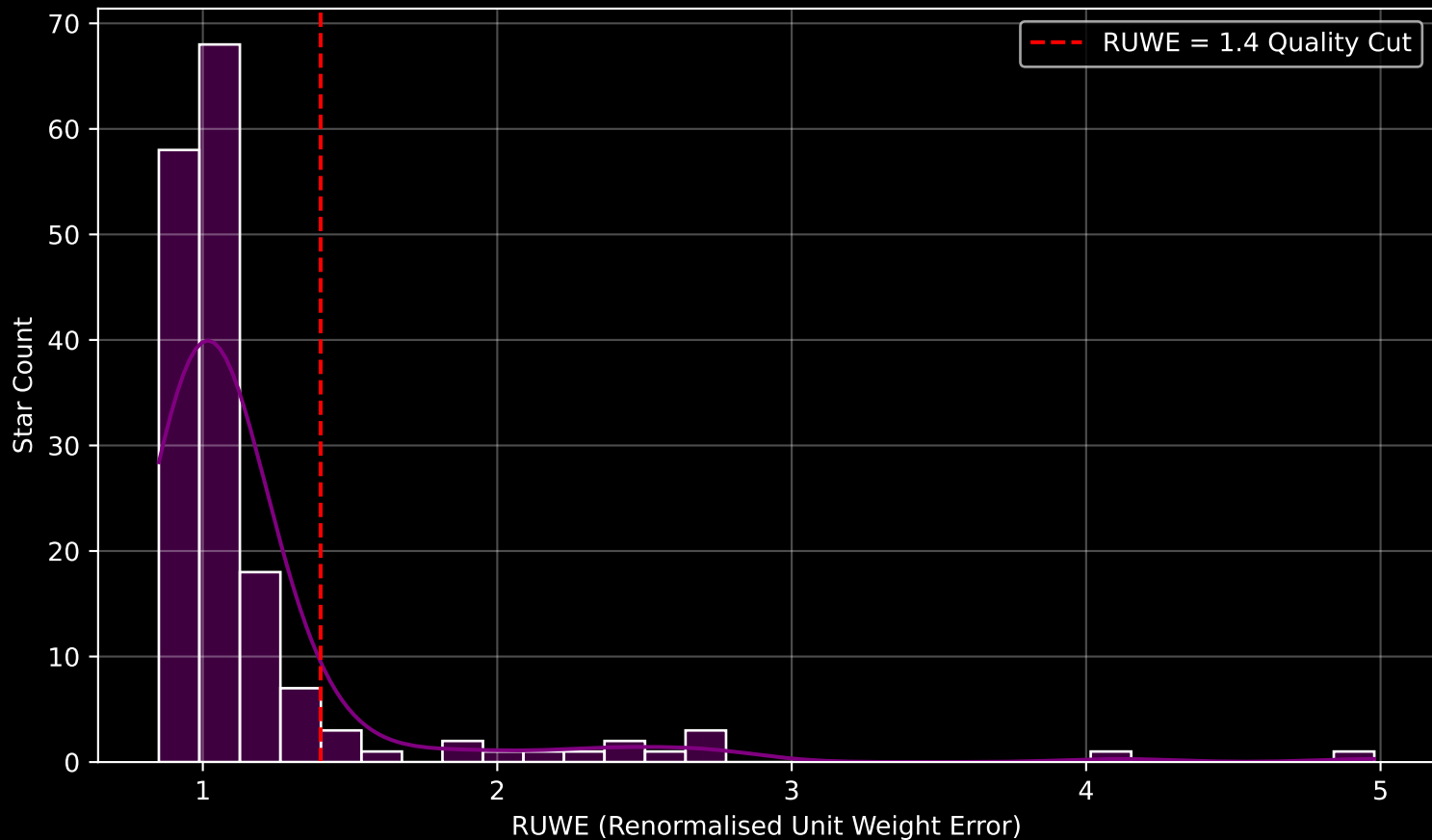
GAPOGEE DR17 Field [TRIAND-3] RUWE Distribution (n= 168)
