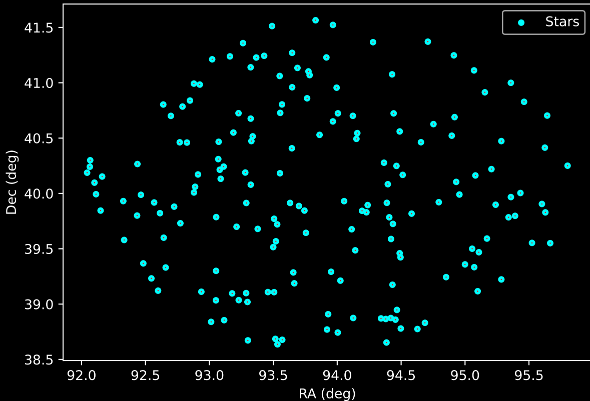
APOGEE DR17 Field: [TRIAND-3] Proper Motion Vectors for Gaia Star Field (n= 174)
