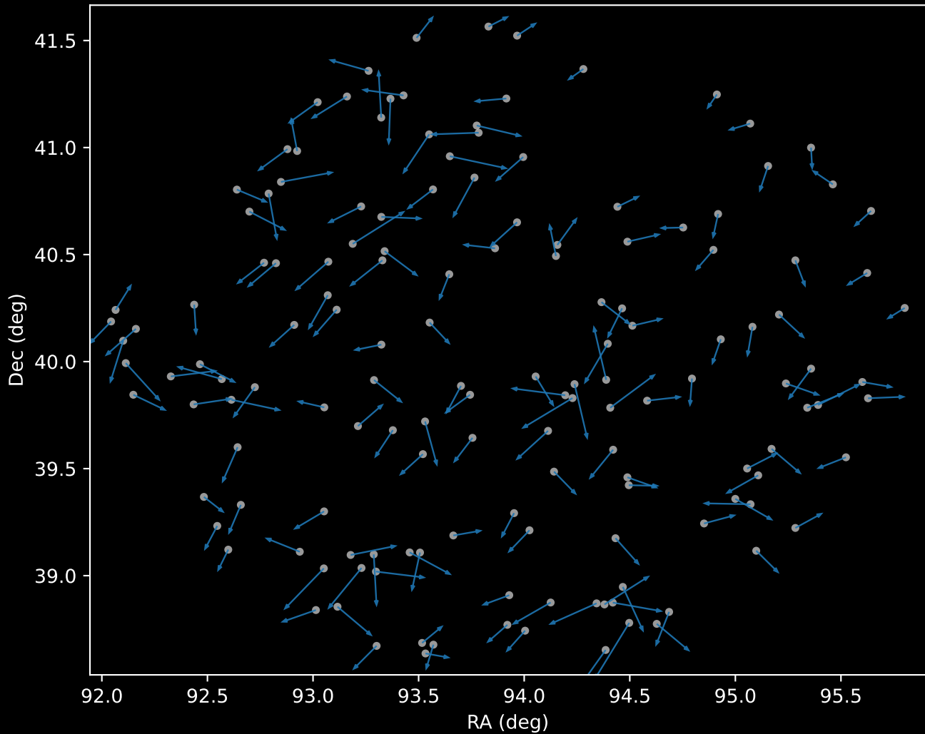
APOGEE DR17 Cluster 0 Proper Motion Vectors (n=149)
